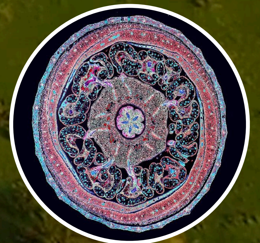
Eukaryotic Cell
