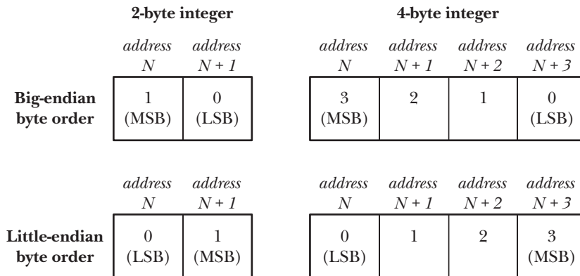
Figure 59-1: Big-endian and little-endian byte order for 2-byte and 4-byte integers
