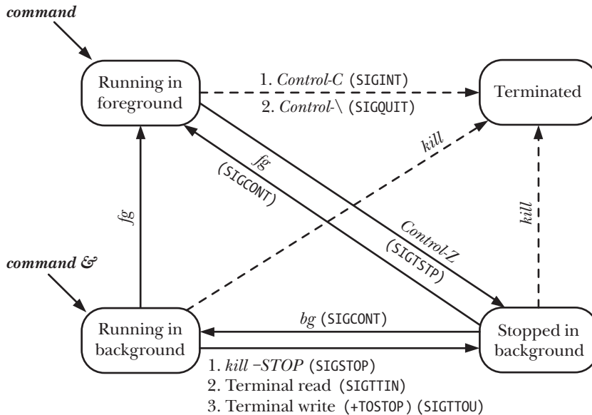
Figure 34-2: Job-control states
