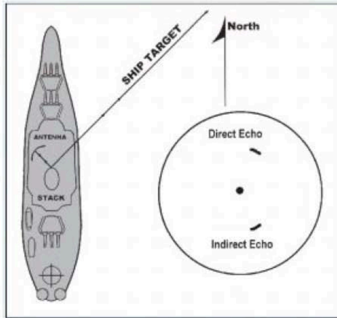
Figure 1307a. Indirect echo.
