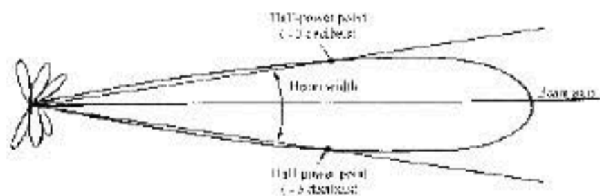
Figure 1303b. Radiation diagram.
