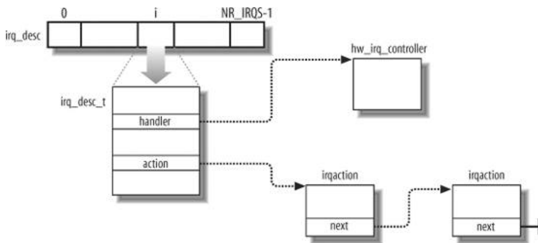
Figure 4-5. IRQ descriptors
