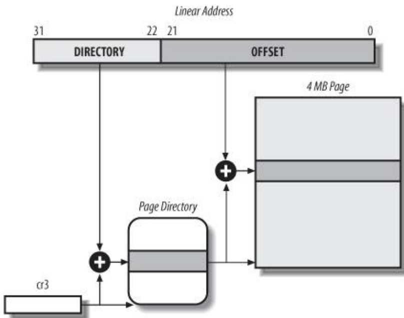
Figure 2-8. Extended paging
