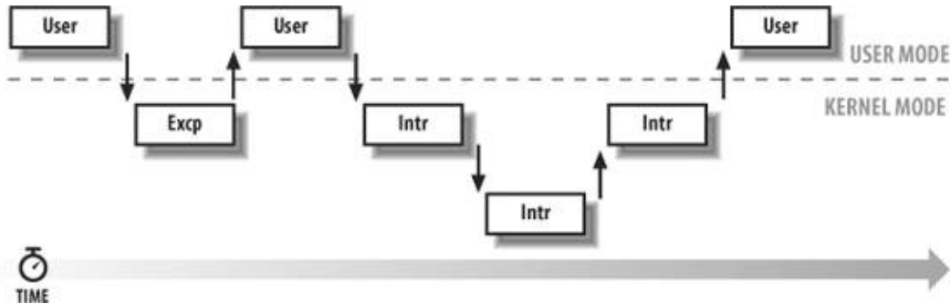
Figure 1-3. Interleaving of kernel control paths
