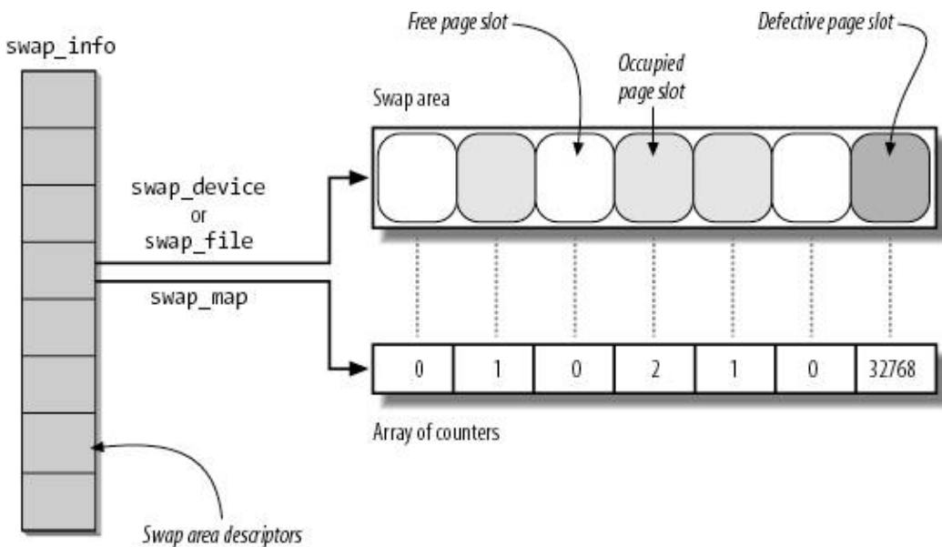
Figure 17-6. Swap area data structures
