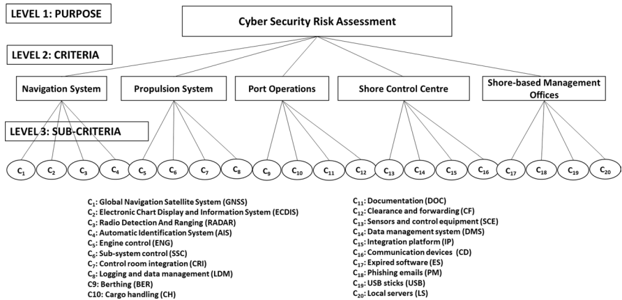
Fig. 1 Cyber security risk assessment framework for autonomous shipping
