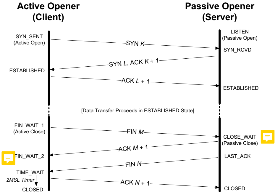
Figure 13-9 TCP states corresponding to normal connection establishment and termination
