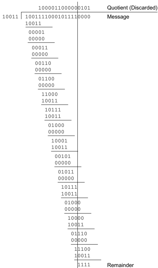
Figure 3-4 Long (mod-2) binary division demonstrating the computation of a CRC4
