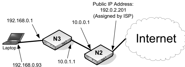
Figure 8-11 The traceroute tool can be used to determine the routing path, assuming it does not fluctuate too quickly. When using traceroute, routers are typically identified by the IP addresses assigned to the interfaces “facing” or nearest to the host performing the trace.
