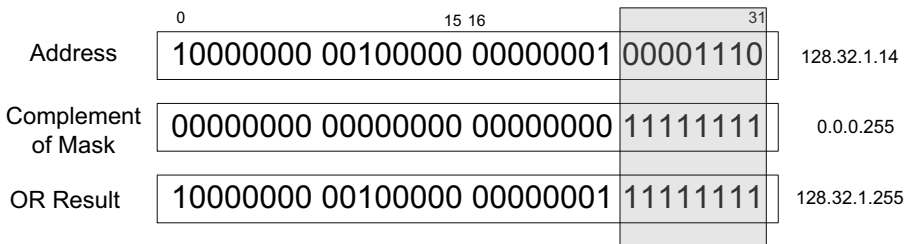
Figure 2-6 The subnet broadcast address is formed by ORing the complement of the subnet mask with the IPv4 address. In this case of a /24 subnet mask, all of the remaining 32 - 24 = 8 bits are set to 1, giving a decimal value of 255 and the subnet broadcast address of 128.32.1.255.
