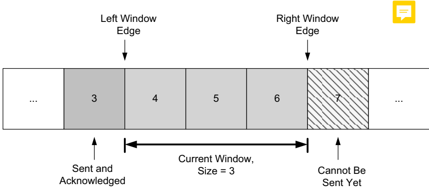
Figure 12-1 The sender’s window, showing which packets are eligible to be sent (or have already been sent), which are not yet eligible, and which have already been sent and acknowledged. In this example, the window size is fixed at three packets.
