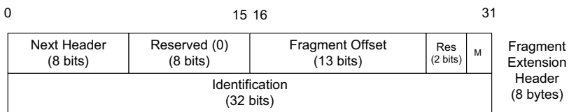
Figure 5-11 The IPv6 Fragment header contains a 32-bit Identification field (twice as large as the Identification field in IPv4). The M bit field indicates whether the fragment is the last of an original datagram. As with IPv4, the Fragment Offset field gives the offset of the payload into the original datagram in 8-byte units.
