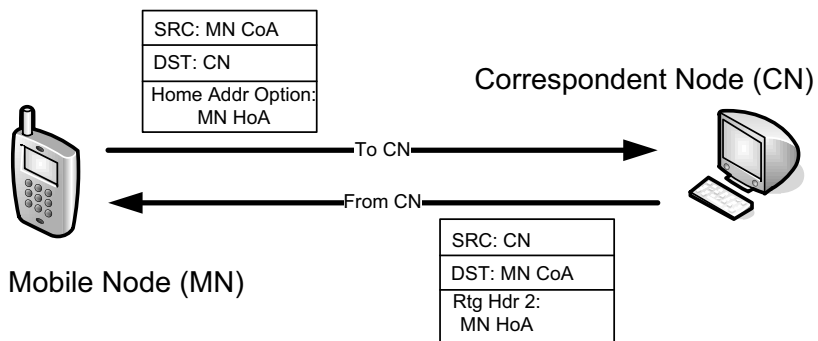
Figure 5-19 Once a binding is established between an MN and a CN, data flows directly between them. The direction from MN to CN uses an IPv6 Home Address Destination option. The reverse direction uses a type 2 Routing header (RH2).
