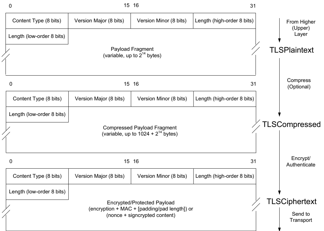
Figure 18-29 The TLS record layer starts with a TLSPplaintext record, which is compressed by a lossless compression algorithm to form a TLSCompressed record. The TLSCompressed record is encrypted (and has a MAC applied) to form a TLSCiphertext record, which is sent for transmission. Conventional stream and block ciphers require a MAC, and block ciphers may include padding. When using AEAD ciphers, a nonce is included with the encrypted and integrity-protected content, but no separate MAC is used.
