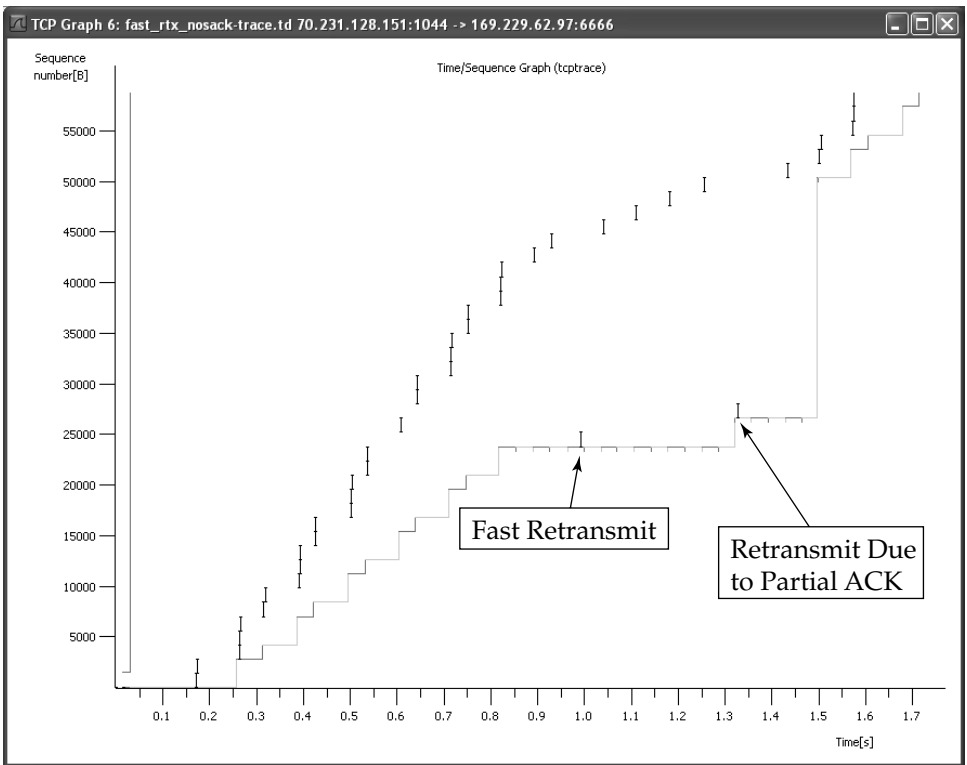
Figure 14-6 In this plot, TCP sequence numbers are on the y-axis and time is on the x-axis. Outgoing segments are displayed as darker line segments, and the incoming ACK numbers appear as lighter gray segments. Fast retransmit is triggered by the arrival of the third duplicate ACK at time 0.993s. This connection does not use SACK, so it is able to repair at most only one hole per RTT. Additional duplicate ACKs arriving after the third cause the sender to send new segments (not retransmissions). A “partial ACK” arriving at time 1.32 causes the next retransmission.
