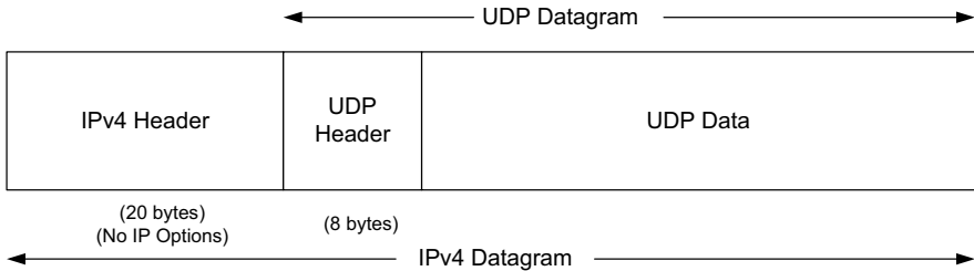
Figure 10-1 Encapsulation of a UDP datagram in a single IPv4 datagram (the typical case with no IPv4 options). The IPv6 encapsulation is similar; the UDP header follows the header chain.
