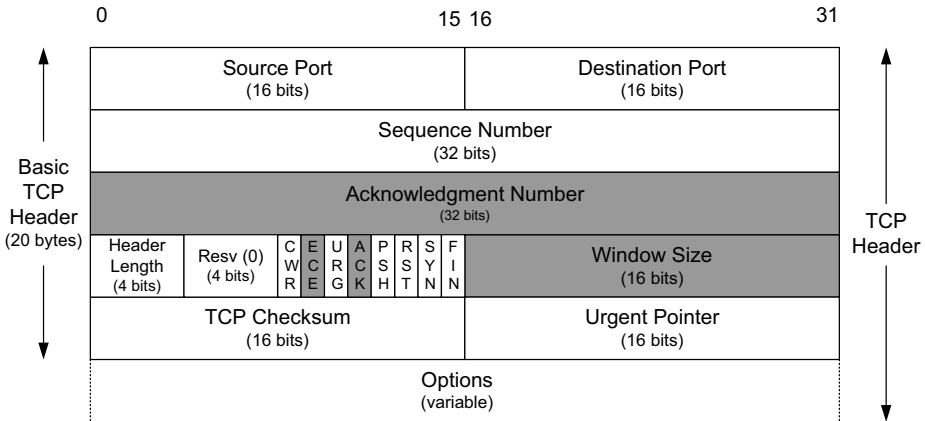
Figure 12-3 The TCP header. Its normal size is 20 bytes, unless options are present. The Header Length field gives the size of the header in 32-bit words (minimum value is 5). The shaded fields (Acknowledgment Number, Window Size, plus ECE and ACK bits) refer to the data flowing in the opposite direction relative to the sender of this segment.
