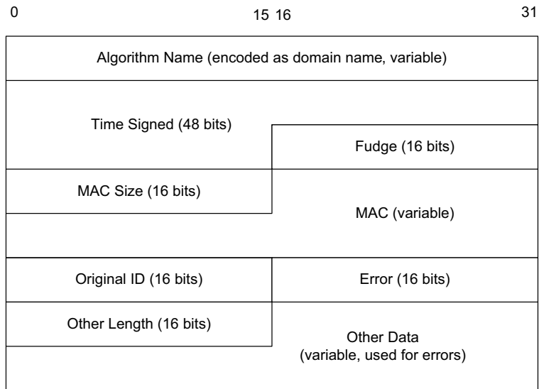
Figure 18-44 The TSIG pseudo-RR RDATA area contains a signature algorithm ID, signature time and time fudge factor, and a MAC. Originally, only an MD5-based signature was used, but now SHA-1- and SHA-2-based signatures have been standardized. TSIG peers must be time-synchronized to within the number of seconds in the Fudge field. TSIG RRs are carried in the additional data section of a DNS message.
