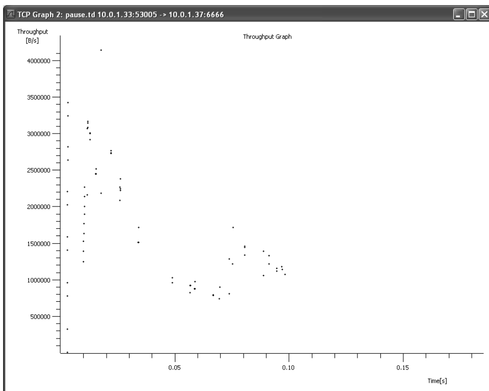
Figure 15-13 With a relatively large receive buffer, a significant amount of data can be transferred even before the receiving application reads any data from the network.
