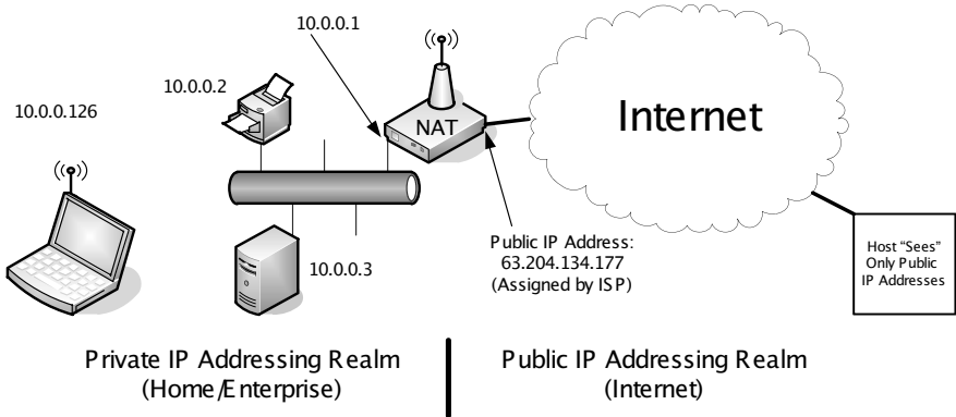
Figure 7-3 A NAT isolates private addresses and the systems using them from the Internet. Packets with private addresses are not routed by the Internet directly but instead must be translated as they enter and leave the private network through the NAT router. Internet hosts see traffic as coming from a public IP address of the NAT.
