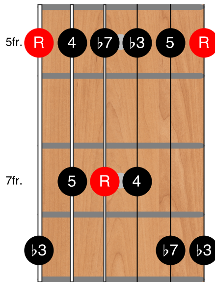
A Minor Pentatonic Scale
