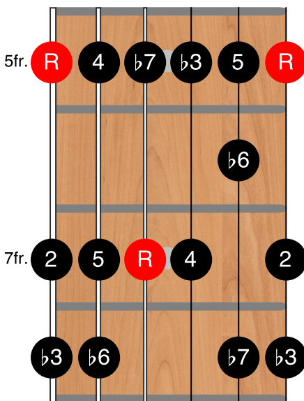
A Aeolian (Natural Minor) Scale
