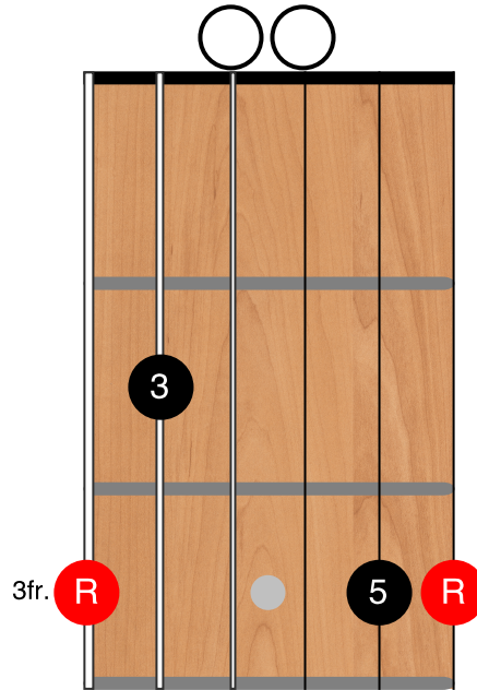
G Major Chord
