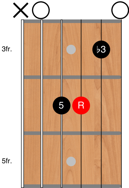
A Minor Chord
