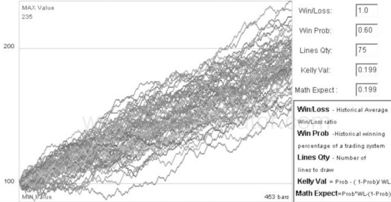
Figure 4.1 Simulated portfolios
