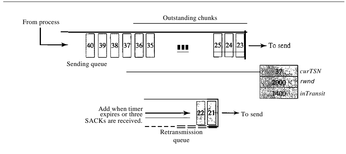
Figure 23.40 Error control, sender site
