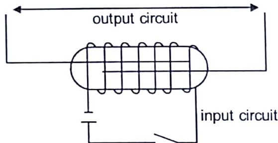
A reed relay
