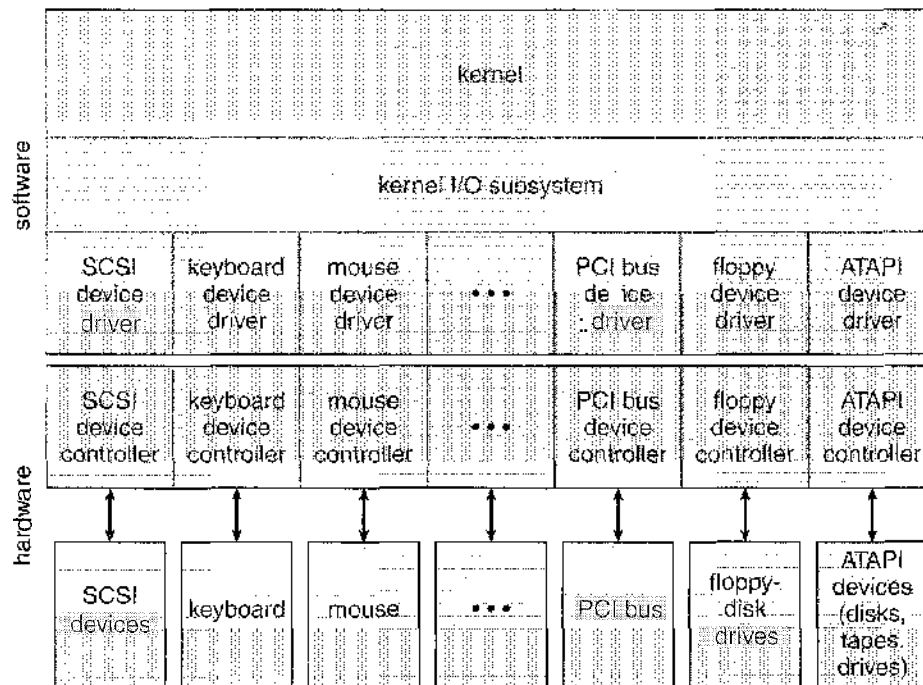
Figure 13.6 A kernel I/O structure.
