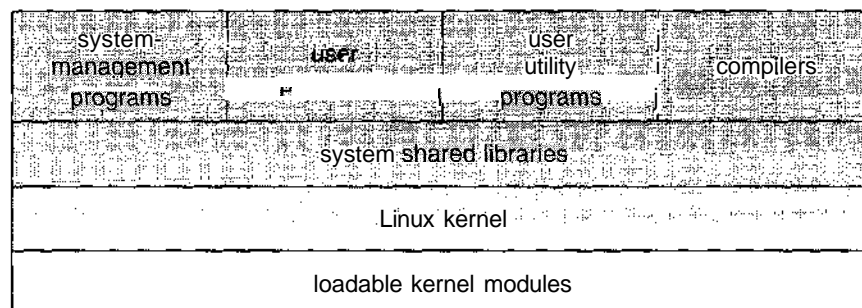
Figure 21.1 Components of the Linux system.
