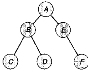
tree-structured network
