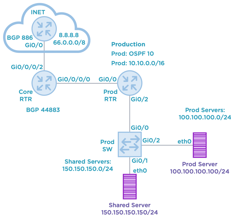
Figure 1 - ZigZagZoo Production Network Diagram
