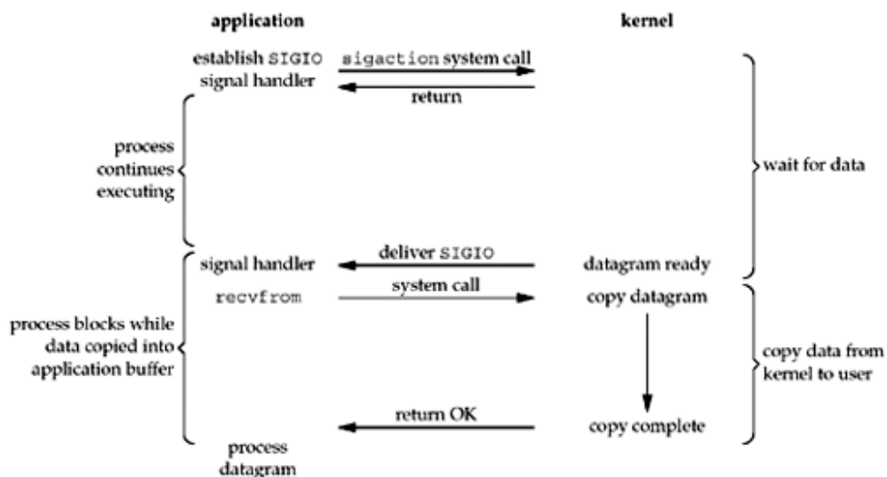
Figure 6.4. Signal-Driven I/O model.
