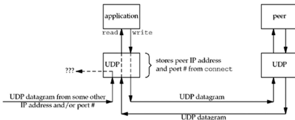
Figure 8.15. Connected UDP socket.
