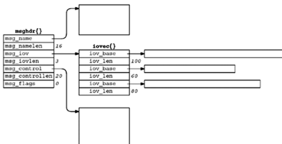
Figure 14.8. Data structures when recvmsg is called for a UDP socket.
