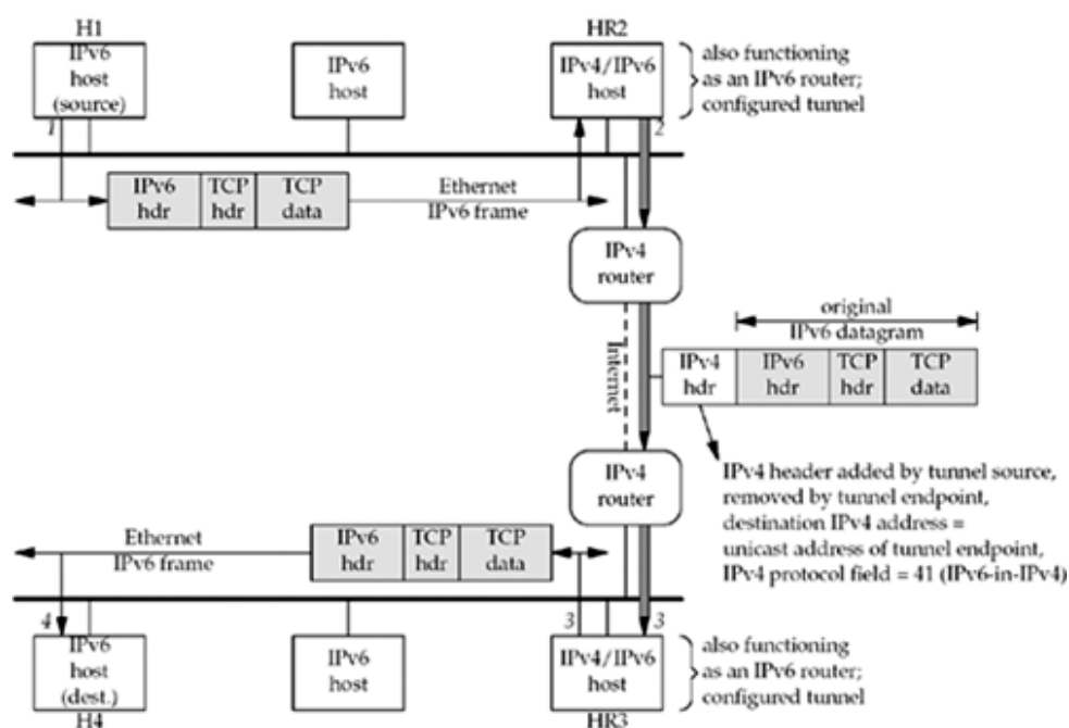
Figure B.2. IPv6-in-IPv4 encapsulation on 6bone.
