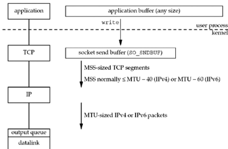
Figure 2.15. Steps and buffers involved when an application writes to a TCP socket.
