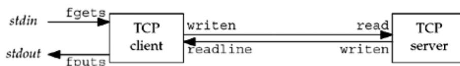
Figure 5.1. Simple echo client and server.
