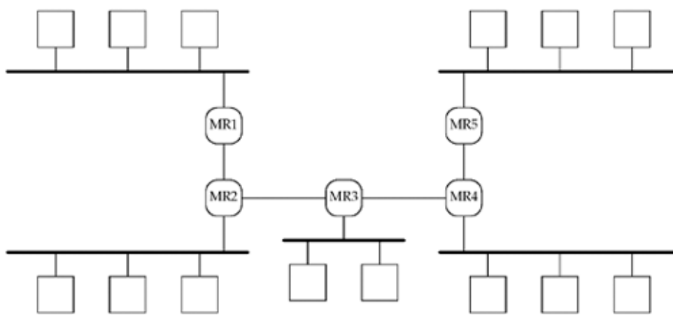
Figure 21.5. Five LANs connected with five multicast routers.
