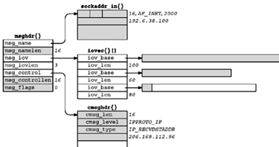
Figure 14.9. Update of Figure 14.8 when recvmsg returns.
