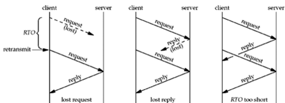
Figure 22.5. Three scenarios when retransmission timer expires.
