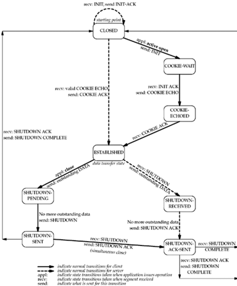
Figure 2.8. SCTP state transition diagram.
