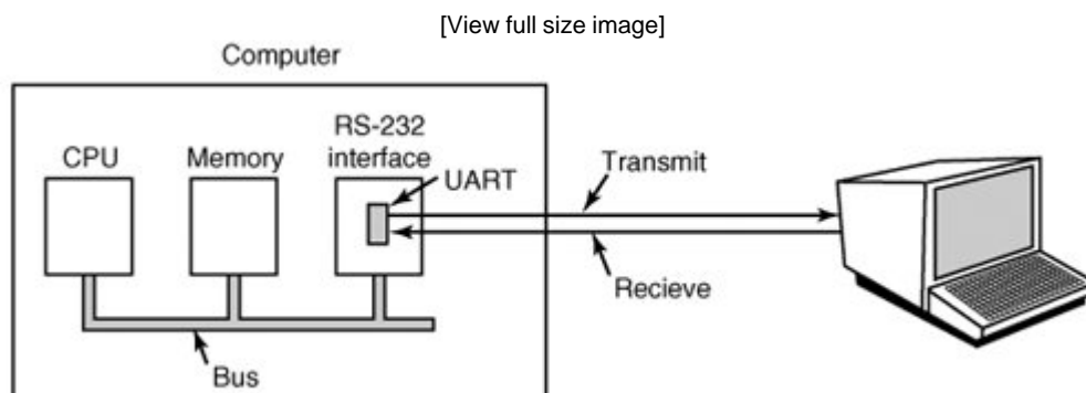
Figure 3-27. An RS-232 terminal communicates with a computer over a communication line, one bit at a time. The computer and the terminal are completely independent.
