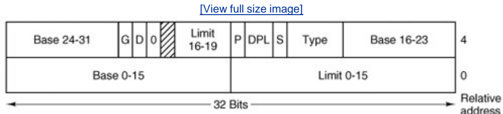
Figure 2-44. The format of an Intel segment descriptor.
