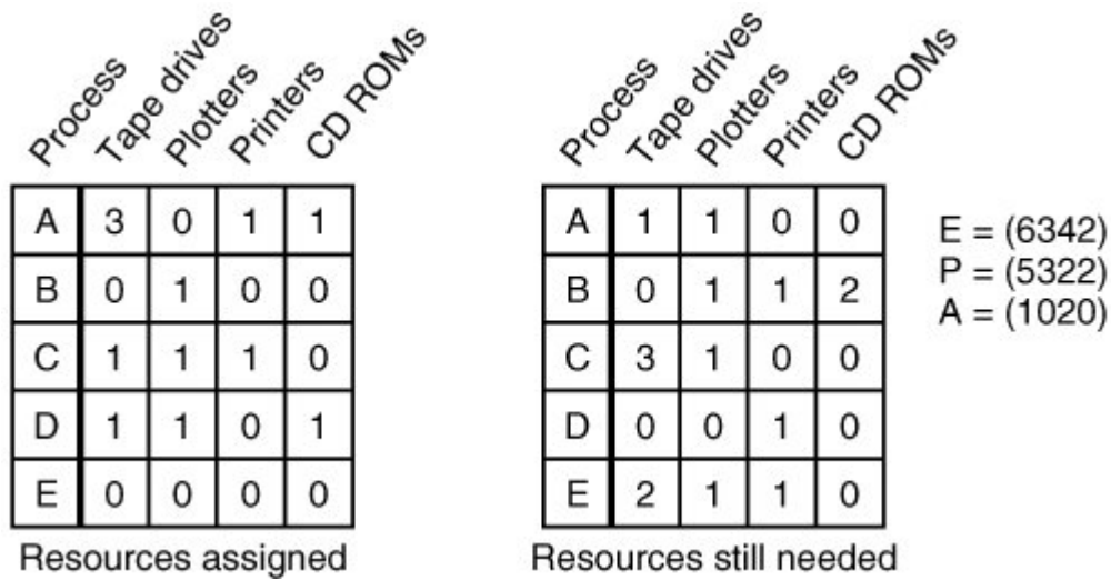
Figure 3-15. The banker's algorithm with multiple resources.
