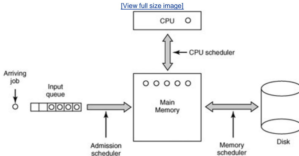
Figure 2-25. Three-level scheduling.
