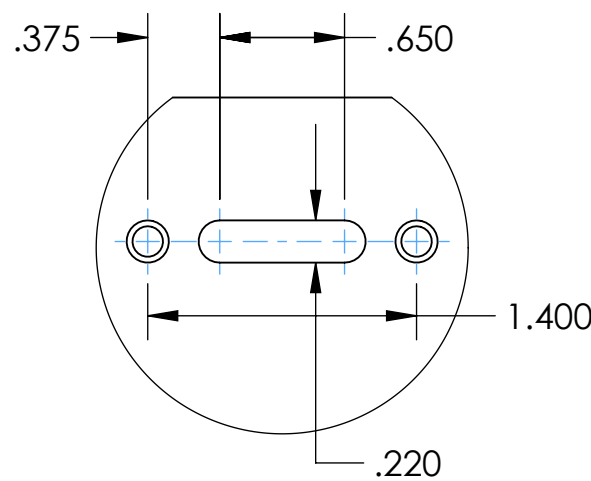
DETAIL B SCALE 1 : 1 3 PLACES
