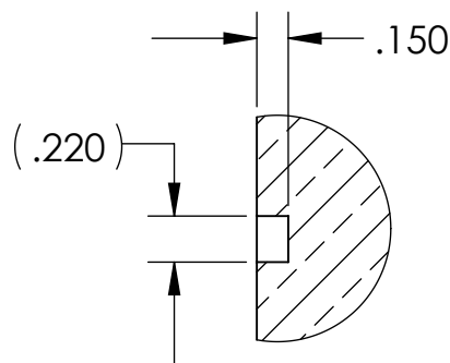
DETAIL C SCALE 1 : 1 3 PLACES
